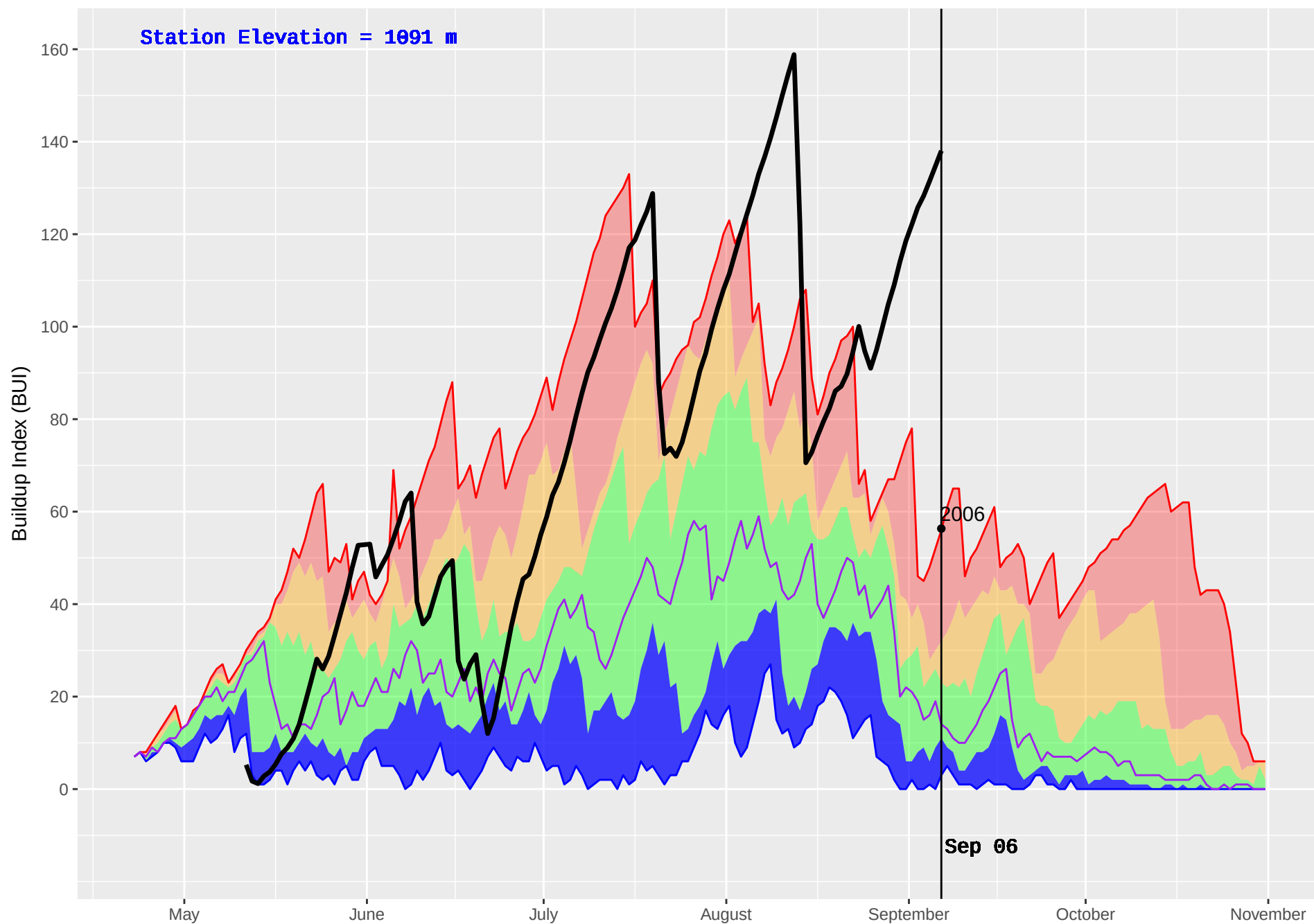
BIG MOUTH 2 (868) : Historical (2004–2016) and Current (2017) Noon Buildup Index (BUI)
